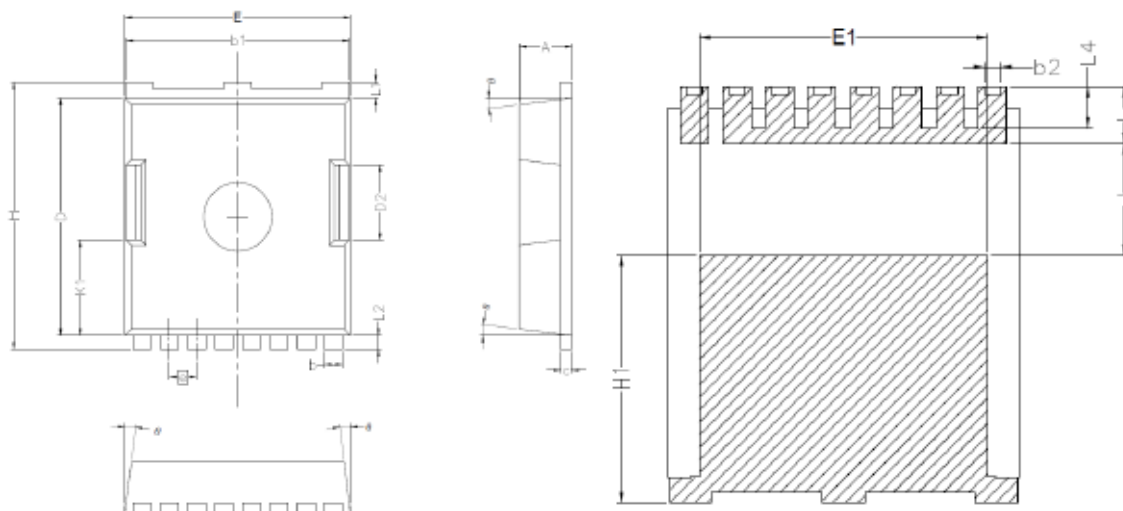
TOLL-8 Package
