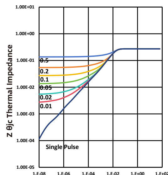
Fig.16 Transient Thermal Impedance
