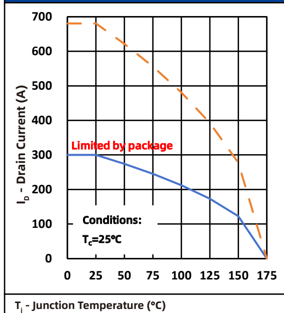
Fig.2 Current Capability
