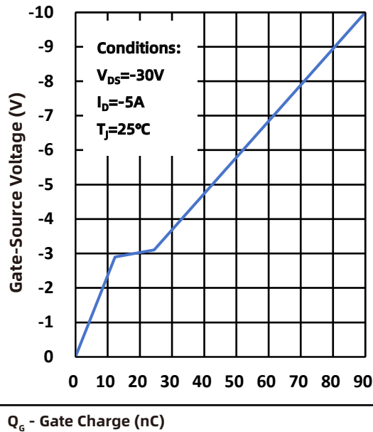
Fig.9 Gate Charge
