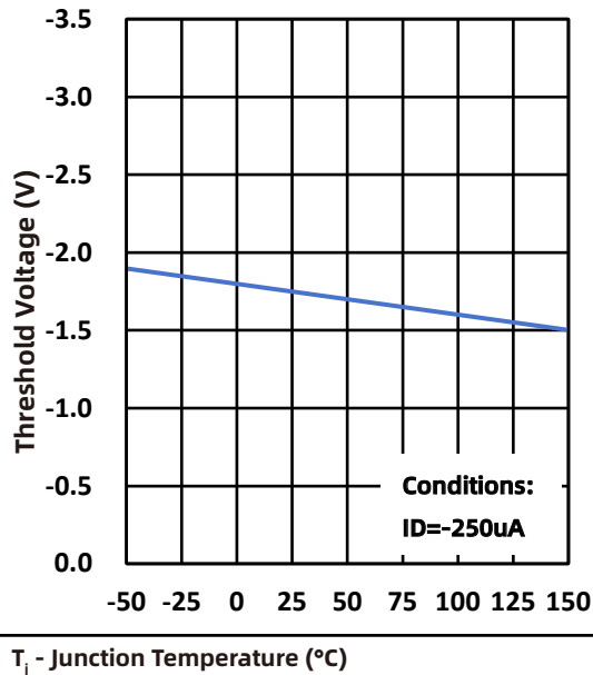
Fig.11 Normalized Threshold Voltage
