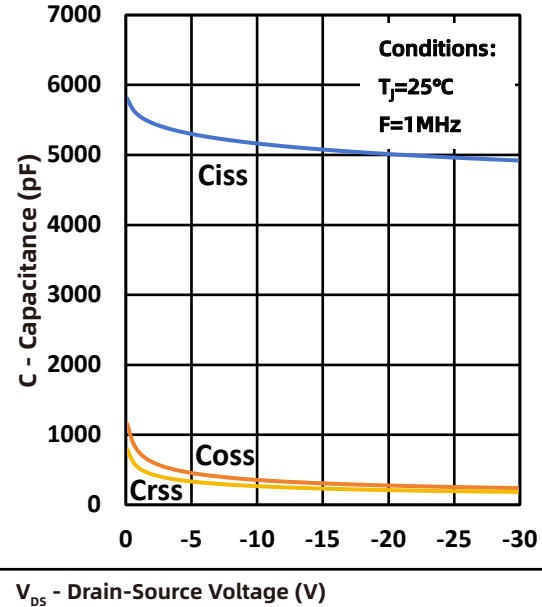
Fig.10 Capacitance
