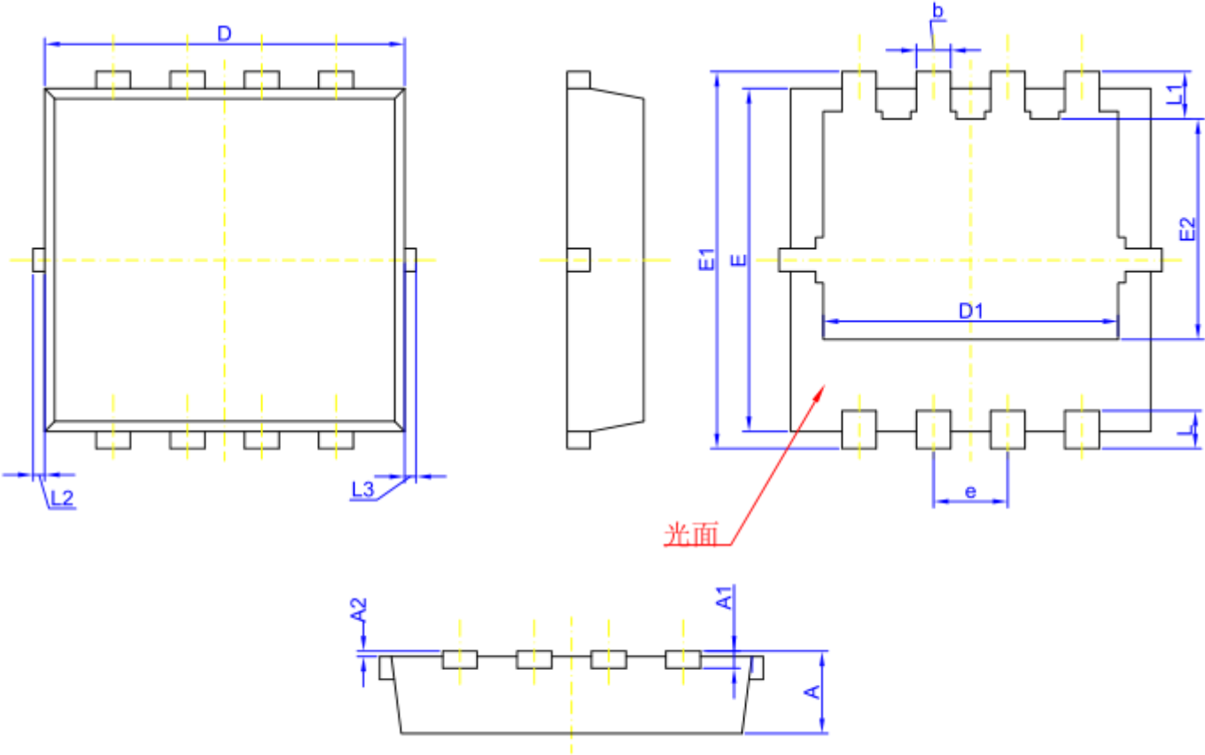
PDFN3.3*3.3 Package
