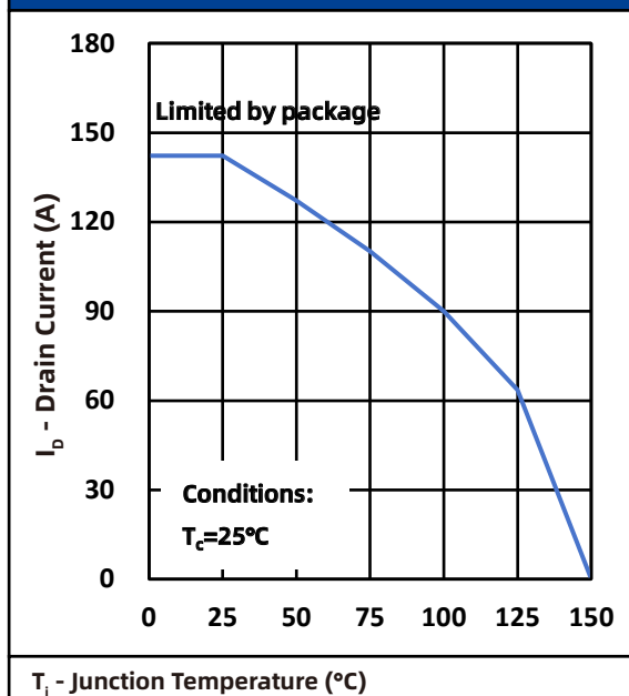
Fig.2 Current Capability
