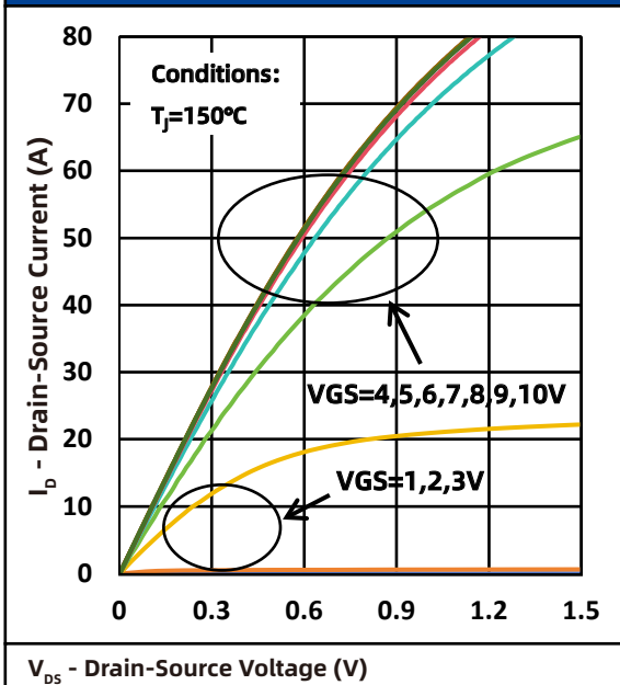
Fig.5 Output Characteristics@Tj 150°C
