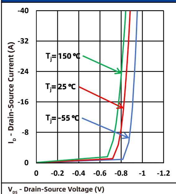
Fig.7 Body Diode Characteristics
