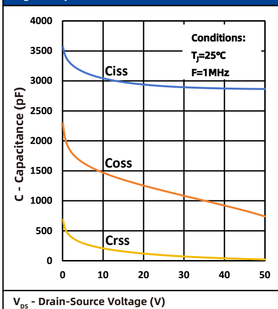
Fig.10 Capacitance
