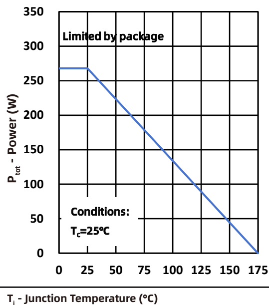
Fig.1 Power Capability
