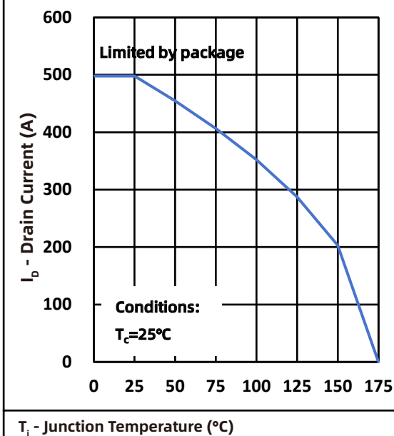
Fig.2 Current Capability
