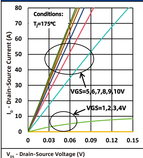
Fig.5 Output Characteristics@Tj 175°C
