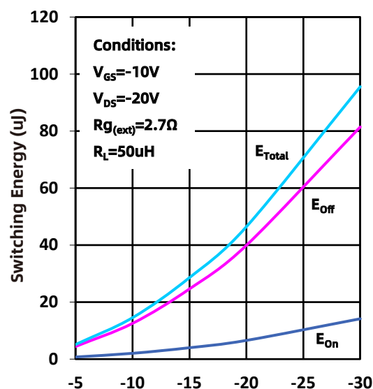
Fig.14 Switching Energy vs I_D
