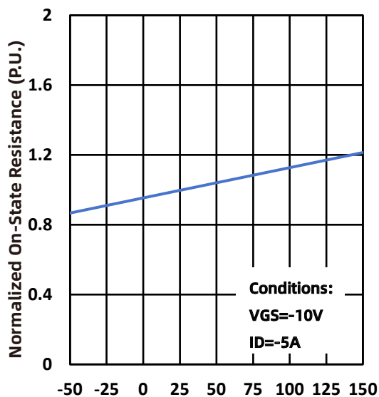
Fig.13 Normalized On Resistance
