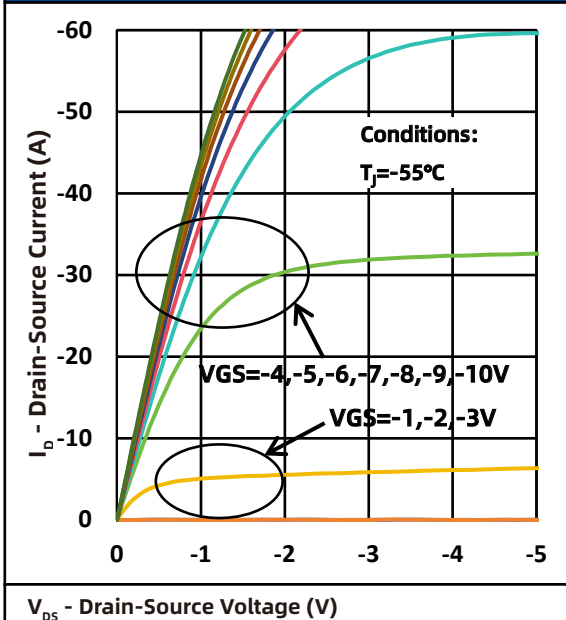
Fig.3 Output Characteristics@Tj -55°C
