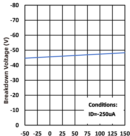
Fig.12 Normalized Breakdown Voltage
