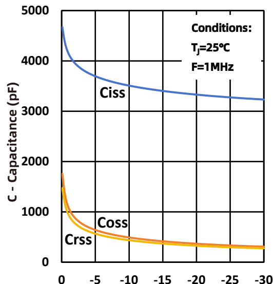
Fig.10 Capacitance
