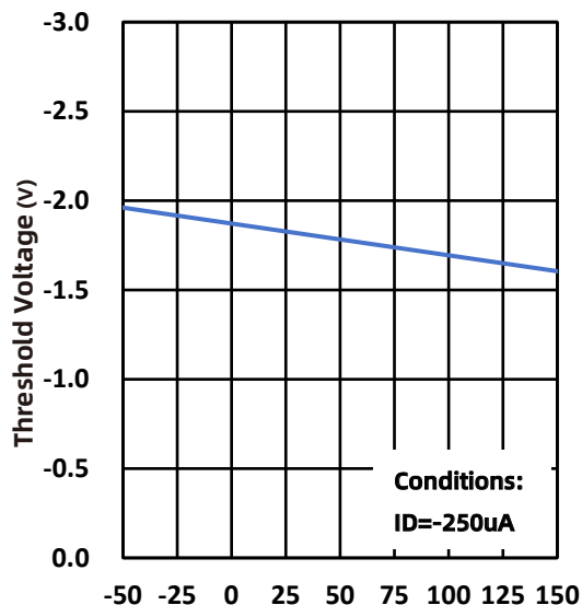
Fig.11 Normalized Threshold Voltage
