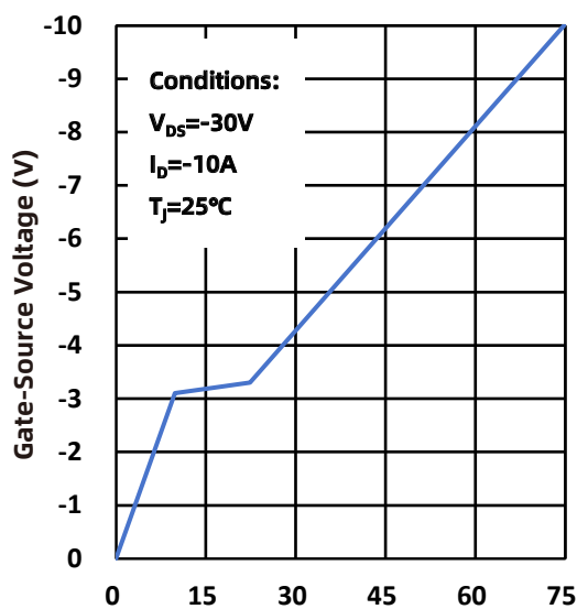
Fig.9 Gate Charge
