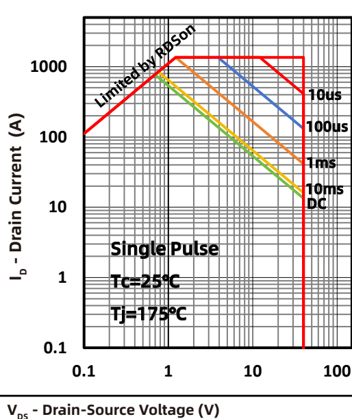
Fig.15 Safe Operating Area
