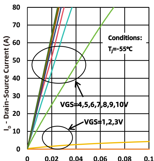
Fig.3 Output Characteristics@ T_j = -55^\circ\text{C}
