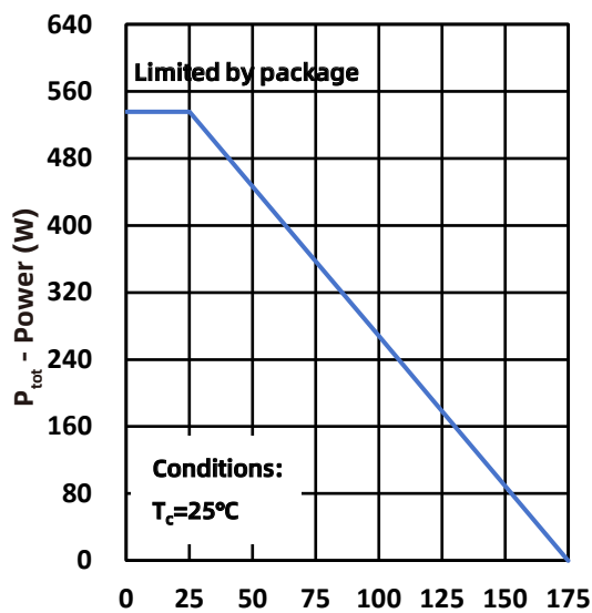
Fig.1 Power Capability
