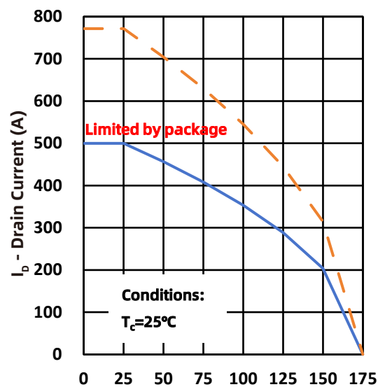
Fig.2 Current Capability
