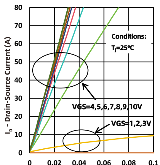
Fig.4 Output Characteristics@ T_j = 25^\circ\text{C}
