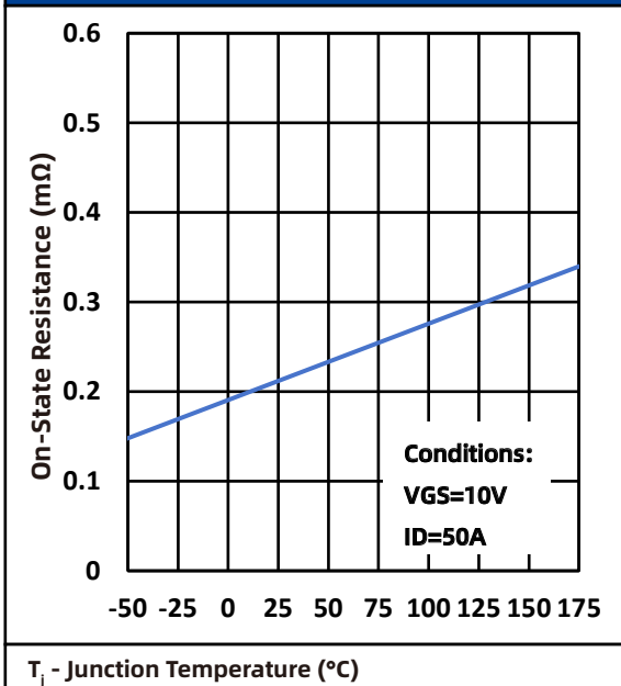
Fig.13 Normalized On Resistance
