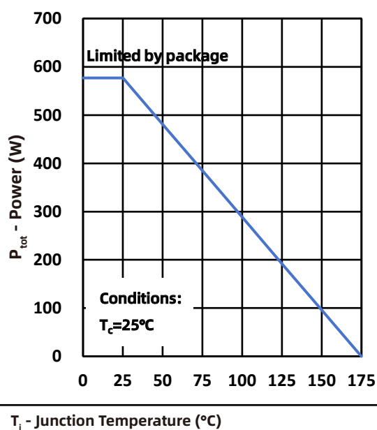
Fig.1 Power Capability
