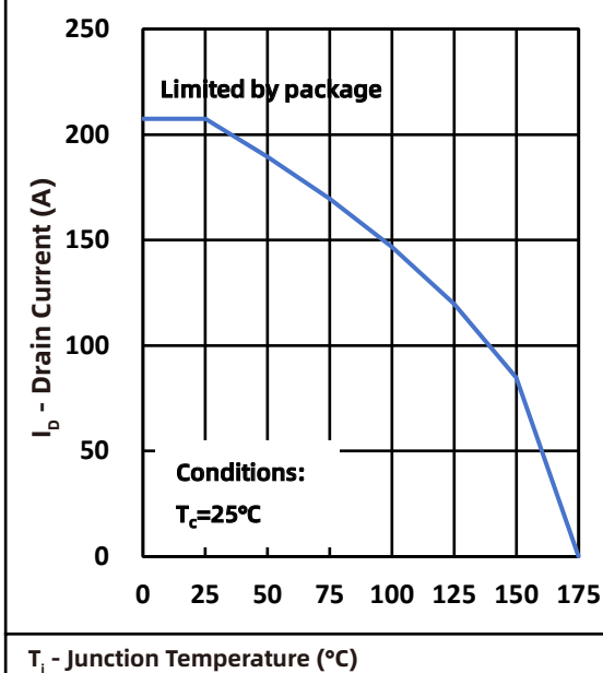
Fig.2 Current Capability
