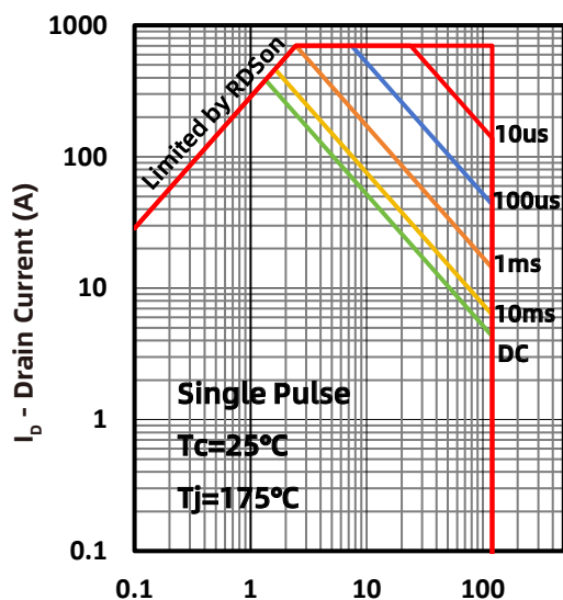
Fig.15 Safe Operating Area
