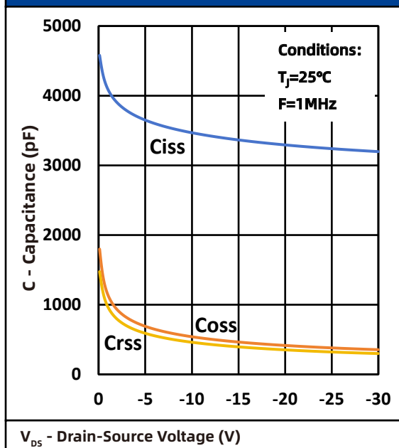
Fig.10 Capacitance
