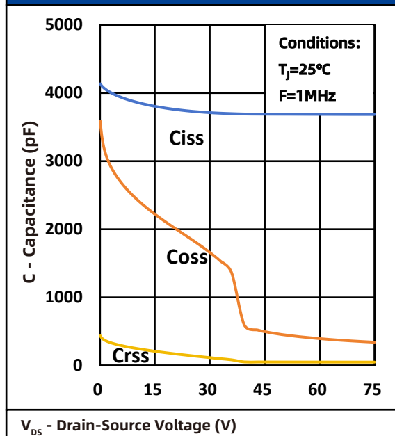
Fig.10 Capacitance
