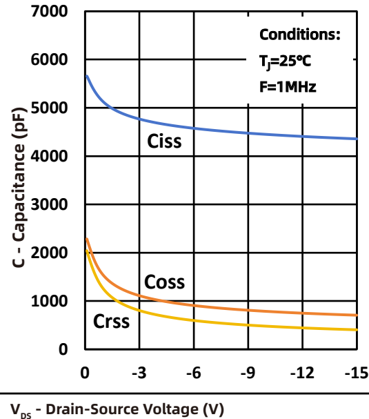
Fig.10 Capacitance
