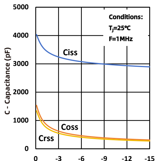
Fig.10 Capacitance
