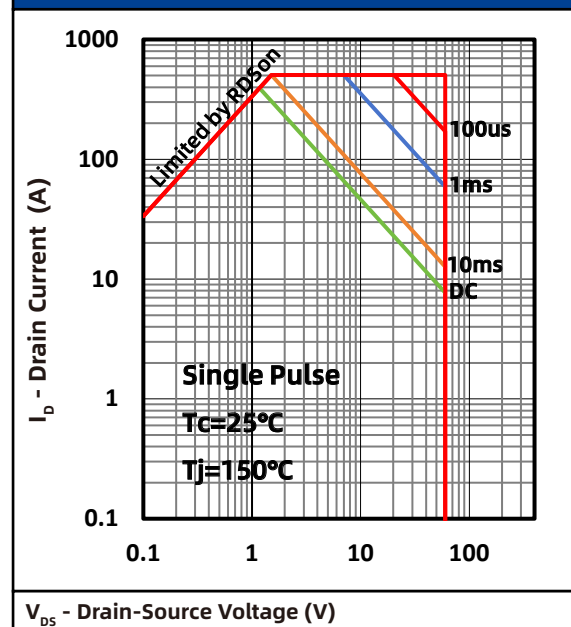
Fig.15 Safe Operating Area
