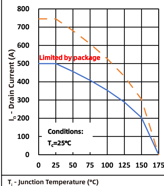
Fig.2 Current Capability
